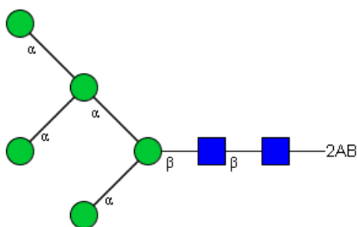
CFG Notation
