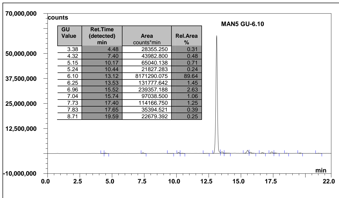
Figure 1: HILIC HPLC profile of 2AB labelled MAN5 glycan (see method conditions below) (Cat. #: CAB-MAN5-01, Batch B37U-01).
