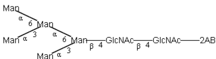
Text Notation
