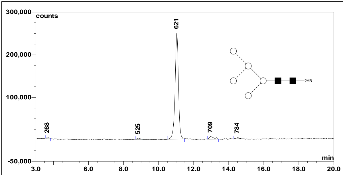
Figure 1: LudgerSepN2 HPLC profile of 2AB labeled MAN 5 glycan (Cat. #: CAB-MAN5-01, Batch B17E-03).
