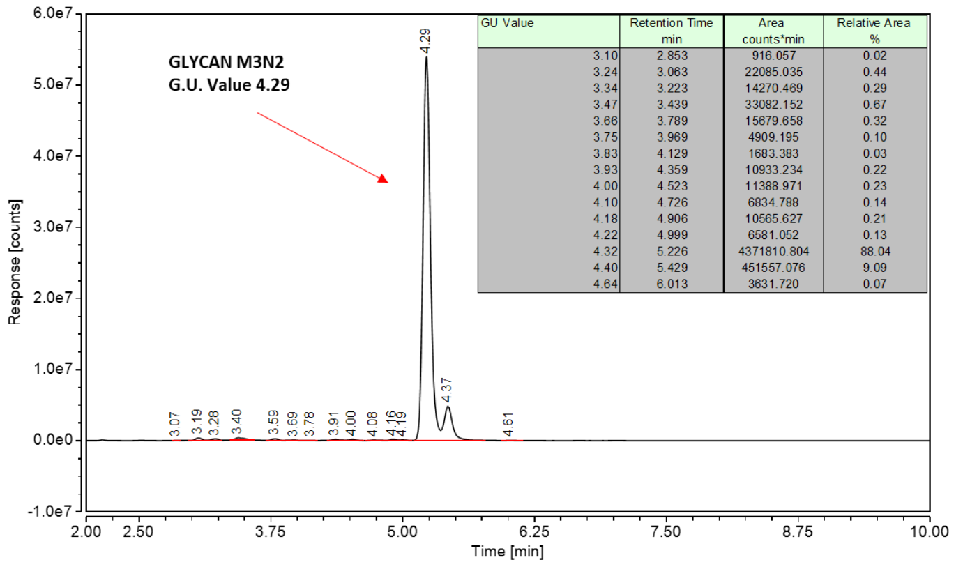
Figure 1: HILIC HPLC profile of 2AB labelled M3N2 glycan (see method conditions below) (Cat. #: CAB-M3N2-01, Batch B8AF-01).
