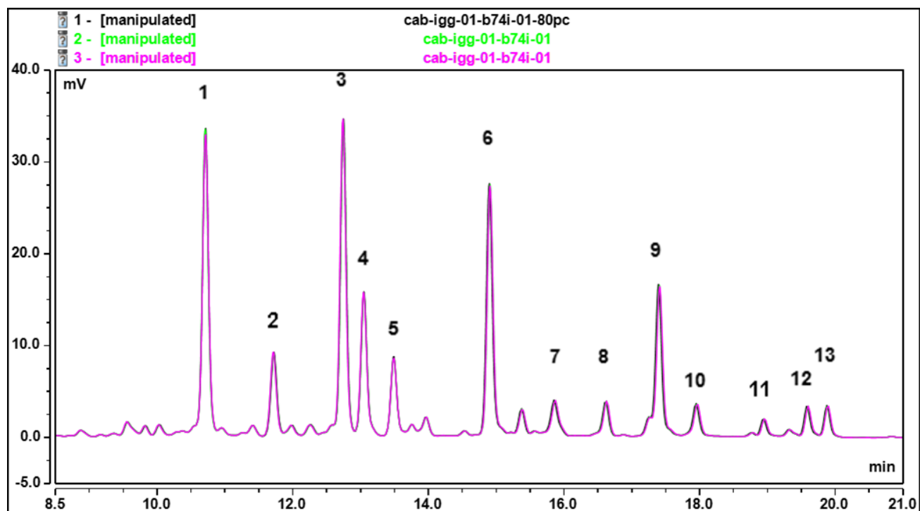
Figure 1: Waters BEH Glycan HPLC Profile of 2AB Labelled IgG N-Glycans, released by N-Mode hydrazinolysis (Cat. No. CAB-IGG-01, Batch B74I-01).
