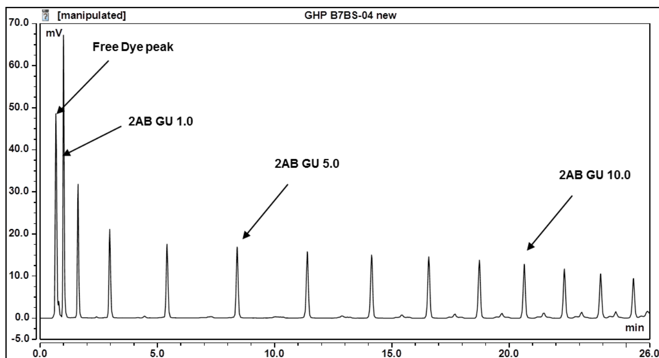
Figure 1: HILIC HPLC profile of 2AB labeled Glucose Homopolymer ladder (Cat. #: CAB-GHP-30, Batch No. B7BS-04).
