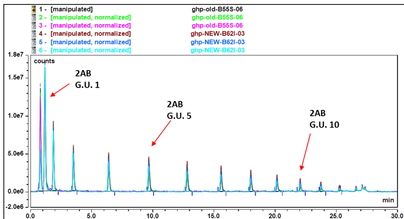
Figure 1 : HILIC HPLC profile of 2AB labeled Glucose Homopolymer ladder (Cat. #: CAB-GHP-30, Batch No. B62I-03 Vs Gold Standard Batch B55S-06).
