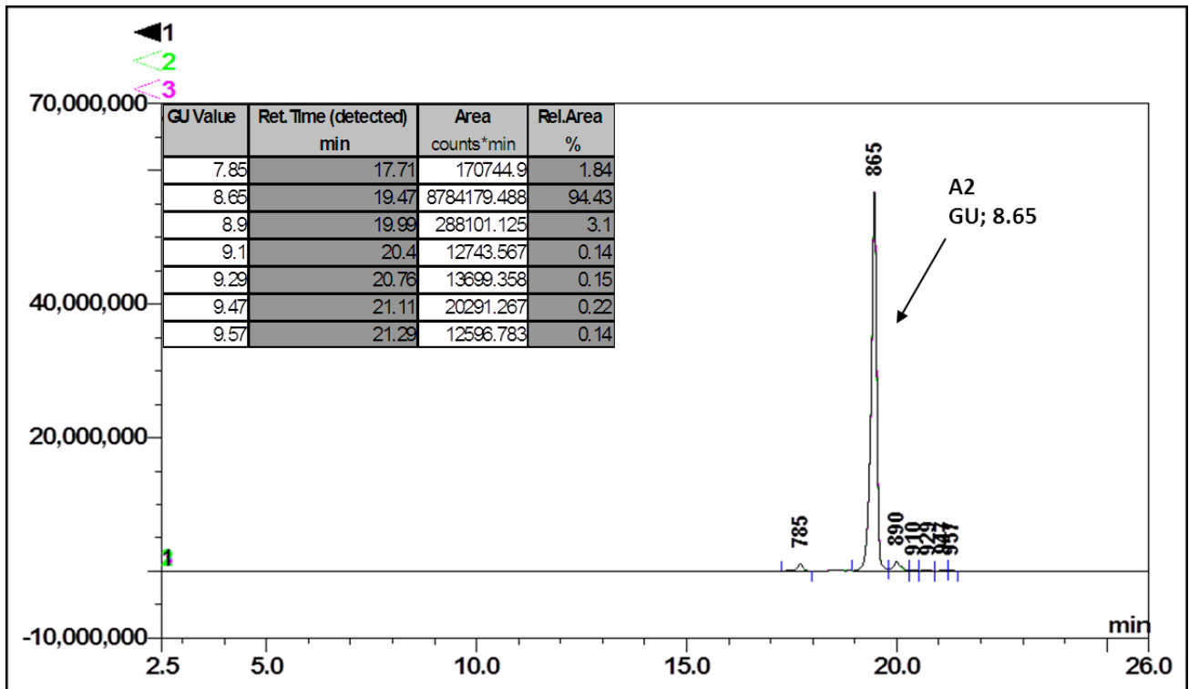
Figure 1: HILIC HPLC profile of 2AB labelled A2 glycan (see method conditions below) (Cat. #: CAB-A2-01, Batch B382-05).
