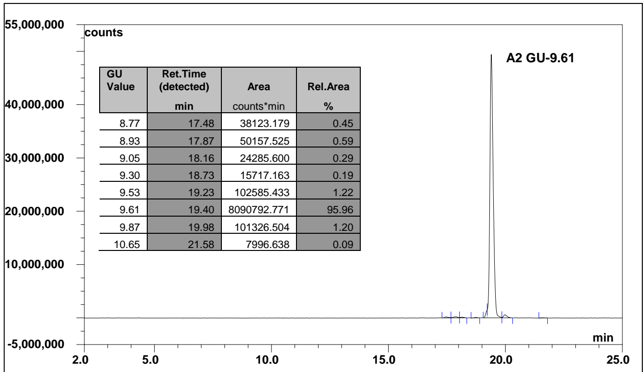
Figure 1: HILIC HPLC profile of 2AB labelled A2 glycan (see method conditions below) (Cat. #: CAB-A2-01, Batch B335-03).
