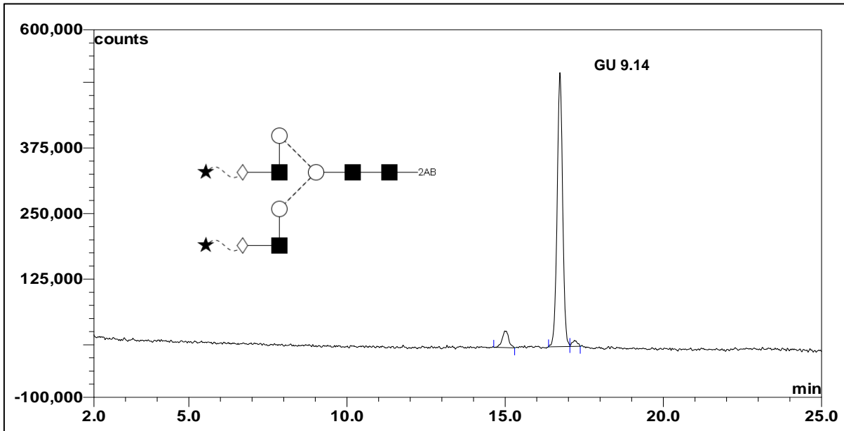
Figure 1: LudgerSepN2 HPLC profile of 2AB labeled A2 glycan (Cat. #: CAB-A2-01, Batch B175-01).
