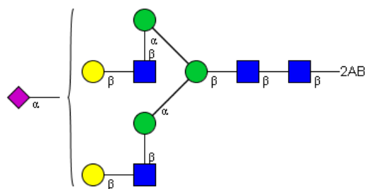
CFG Notation
