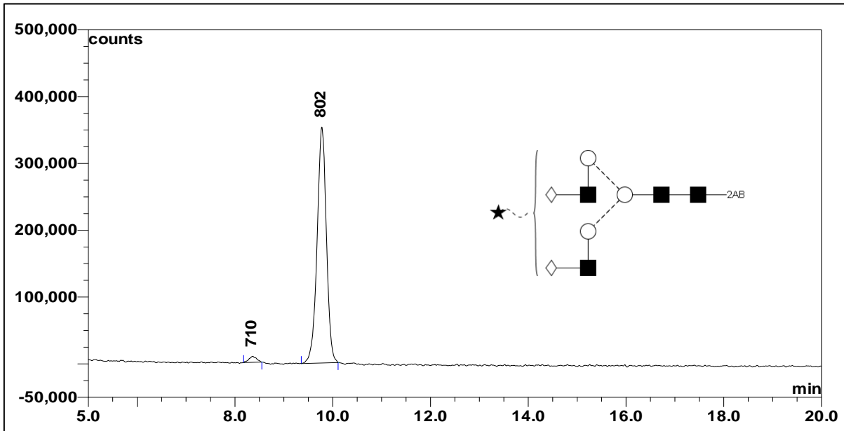
Figure 1: LudgerSepN2 HPLC profile of 2AB labeled A1 glycan (Cat. #: CAB-A1-01, Batch B15D-01).
