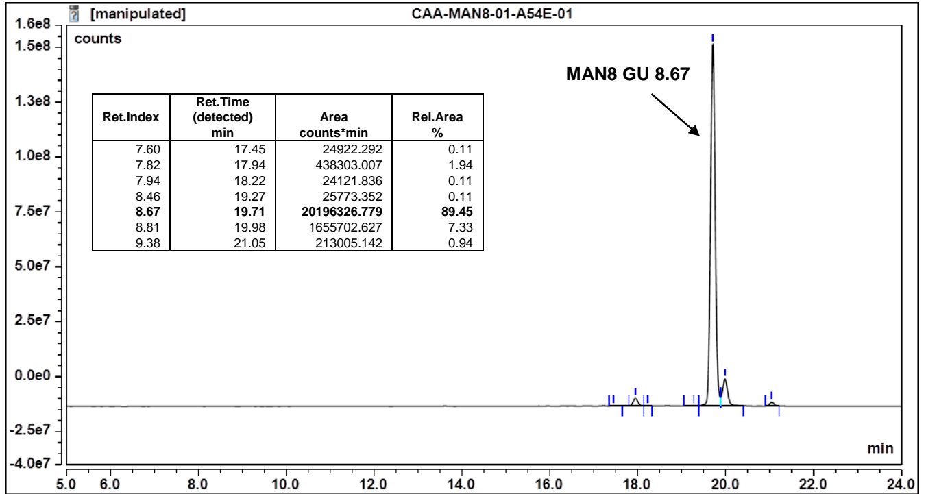
Figure 1: HILIC HPLC profile of 2AA labelled MAN8 glycan (see method conditions below)
