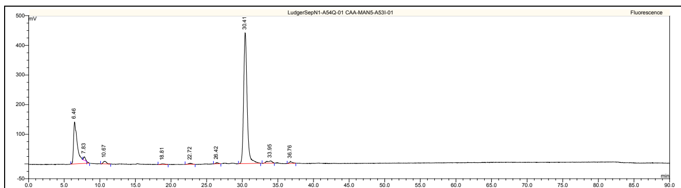
Figure 1 : LudgerSepN1 HPLC profile of 2AA labeled MAN-5 glycan (Cat. #: CAA-MAN5-01, Lot No. A53I-01).
