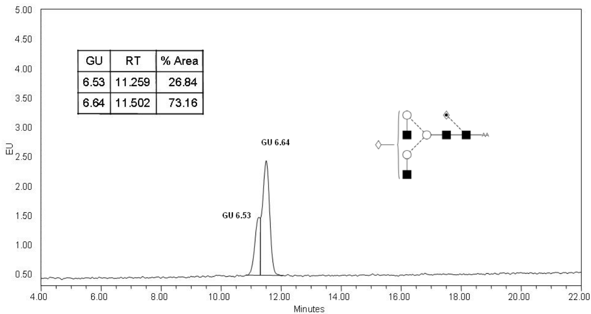
Figure 1 : LudgerSepN2 HPLC profile of 2AA labeled FA2G1 glycan (Cat. #: CAA-FA2G1-01, Batch B08D-01).
