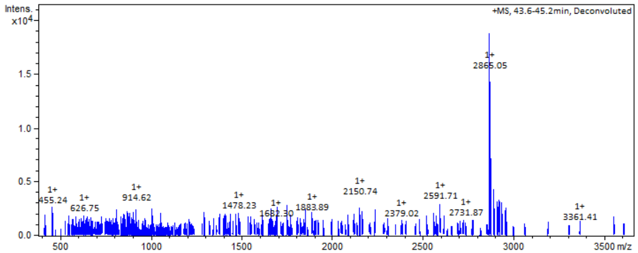
Figure 5. Positive ion ESI mass spectrum of BQ-GPEP-A2G2S2-10U (Batch B74R-01). KVANKT-A2G2S2 theoretical mass: 2865.18 Da;
