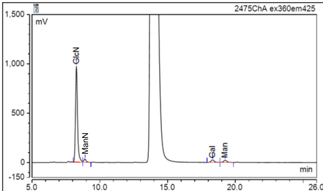
Figure 2. LudgerSep-R2 HPLC profile of 2-aminobenzoic acid (2-AA) labeled monosaccharides of HCl hydrolysed BQ-GPEP-A2G2S2-10U (Batch B74R-01).
