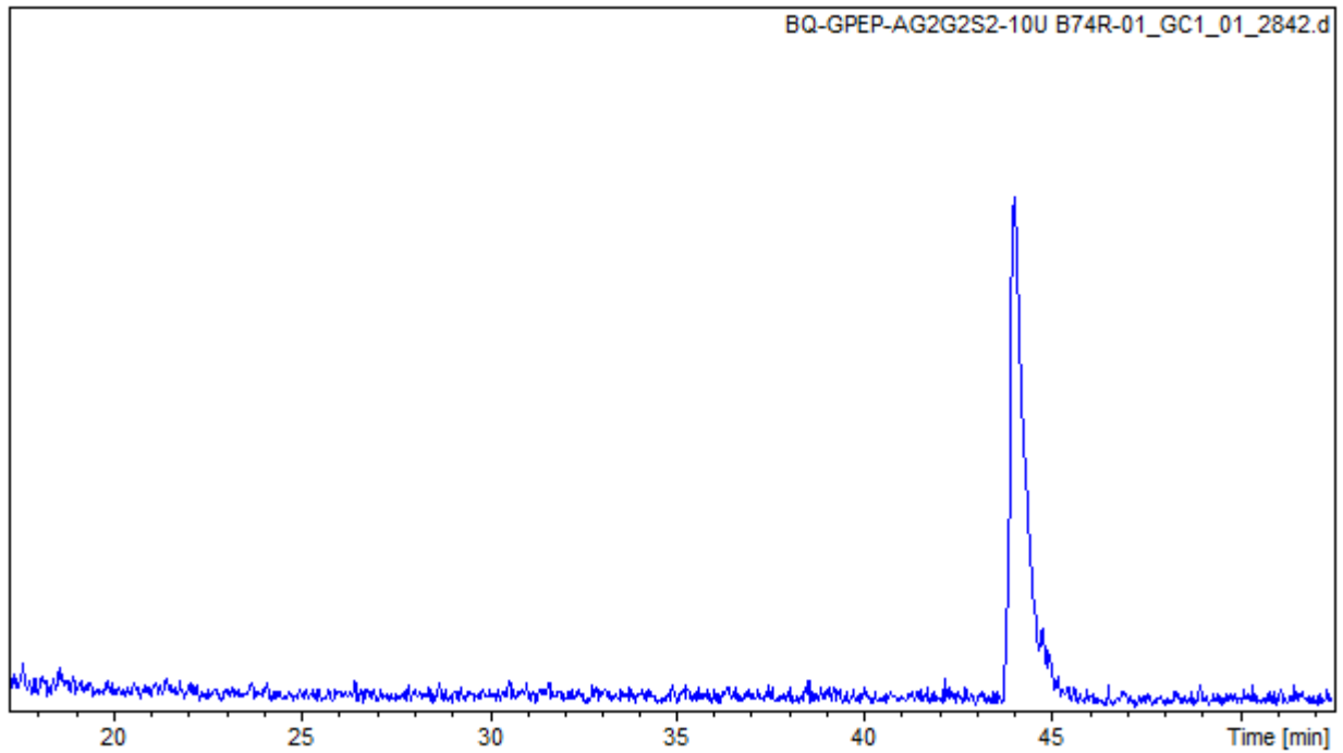
Figure 4. Base Peak Chromatogram-Positive ESI mass spectrum of BQ-GPEP-A2G2S2-10U (Batch B74R-01).
