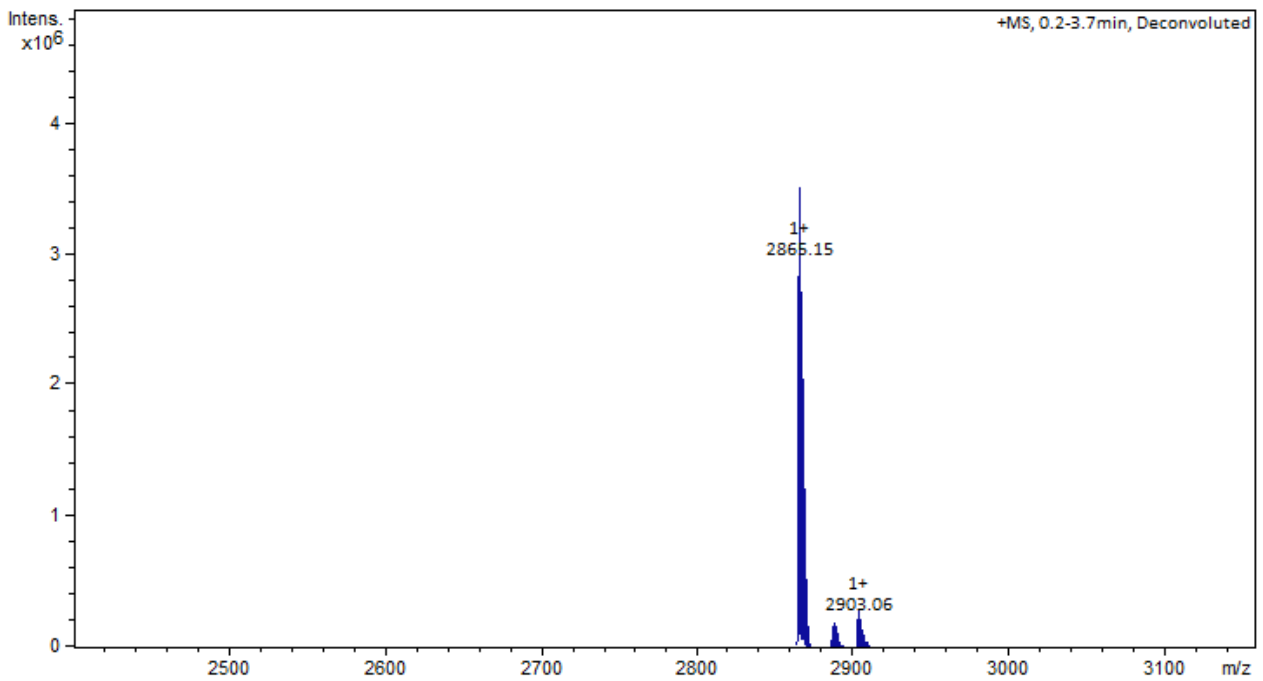
Figure 5. Positive ion ESI mass spectrum of BQ-GPEP-A2G2S2-10U (Batch B68O-03). KVANKT-A2G2S2 theoretical mass: 2865.18 Da
