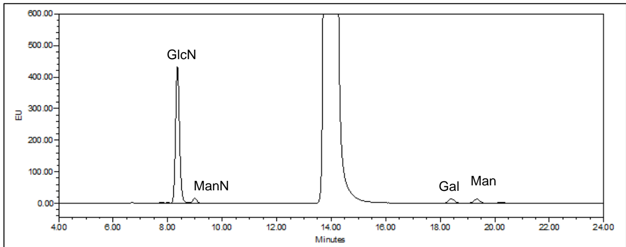
Figure 2. LudgerSep-R2 HPLC profile of 2-aminobenzoic acid (2-AA) labelled monosaccharides of HCl hydrolysed BQ-GPEP-A2G2S2-10U (Batch B68O-03).
