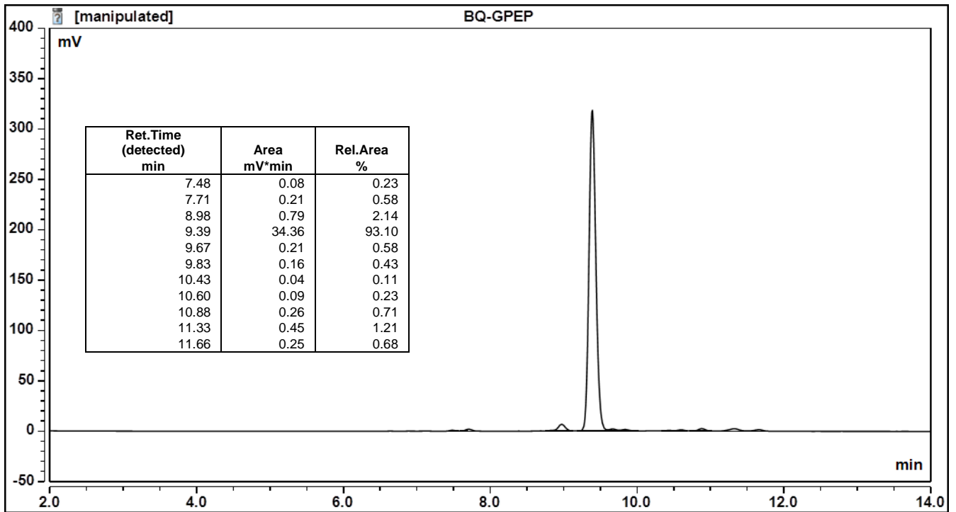
Figure 4. HILIC UHPLC profile of V-Tag (Ludger fluorophore tag) labelled BQ-GPEP-A2G2S2-10U (Batch B68O-03).
