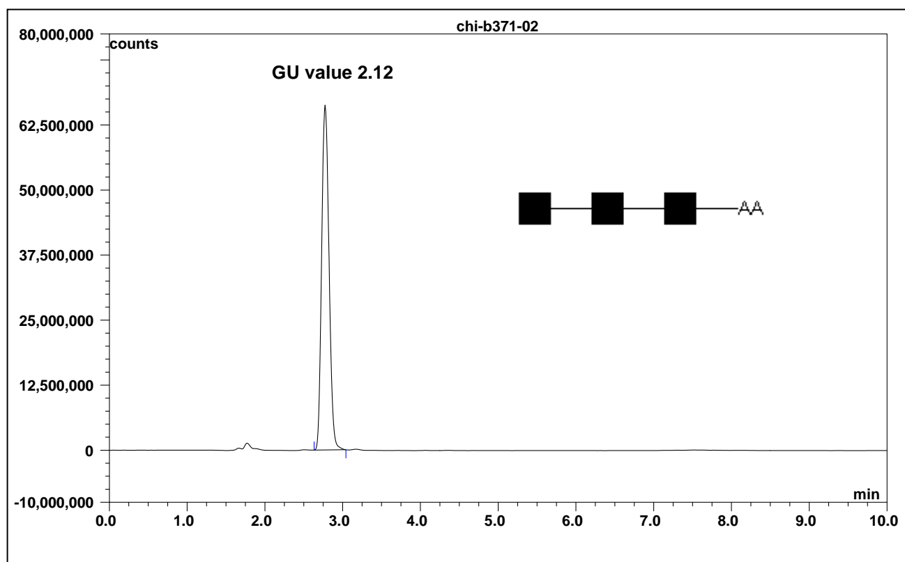
Figure 1: Waters BEH column HPLC profile of 2AA labelled chitotriose standard (Cat. #: BQ-CAA-CHI-01, Batch B37I-02).
