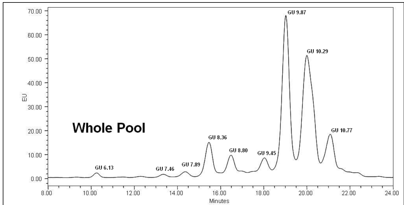
Figure 1: LudgerSepN2 (Cat. #: LS-N2-4.6x150) HPLC profile of 2-AB labelled Fetuin N-glycans, released by PNGase F from GCP-FET-50U batch B04R-03.
