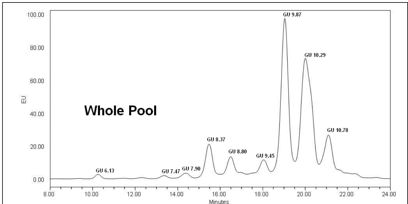
Figure 1: LudgerSepN2 (Cat. #: LS-N2-4.6x150) HPLC profile of 2-AB labelled Fetuin N-glycans, released by PNGase F from GCP-FET-100U batch B06P-01.
