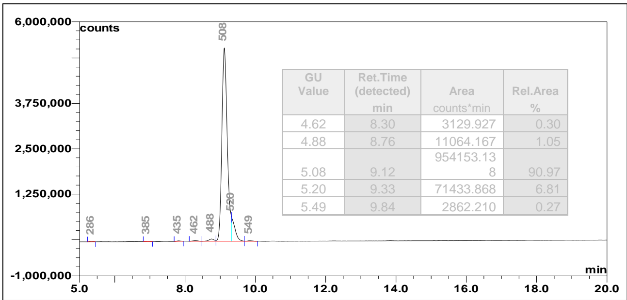
Figure 3: LudgerSepN2 chromatogram of 2AB labelled NGA2 glycan (CN-NGA2-10U, Batch B144-03).
