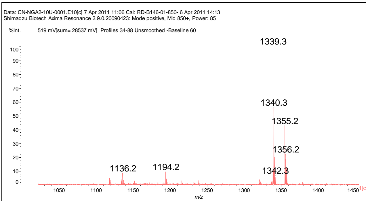
Figure 4: Positive ion mass spectrum of NGA2 glycan (CN-NGA2-10U, Batch B144-03). Theoretical mass 1339.5 Da [M+Na] + .
