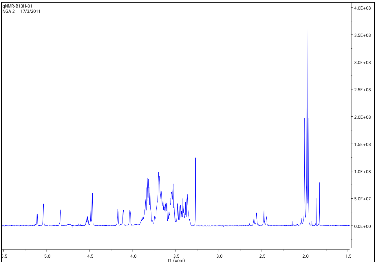
Figure 2: 500MHz 1 H-NMR of NGA2 glycan BULK (CN-NGA2-BULK Batch B148-12).
