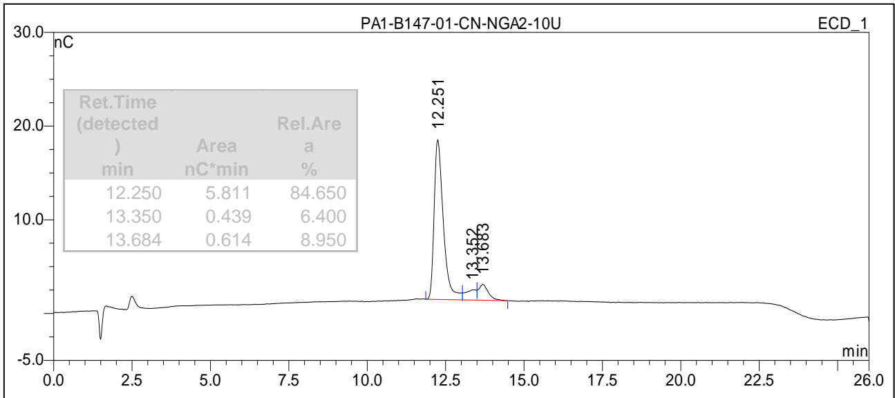
Figure 1 : HPAE-PAD HPLC Profile of NGA2 (CN-NGA2-10U, Batch B144-03).
