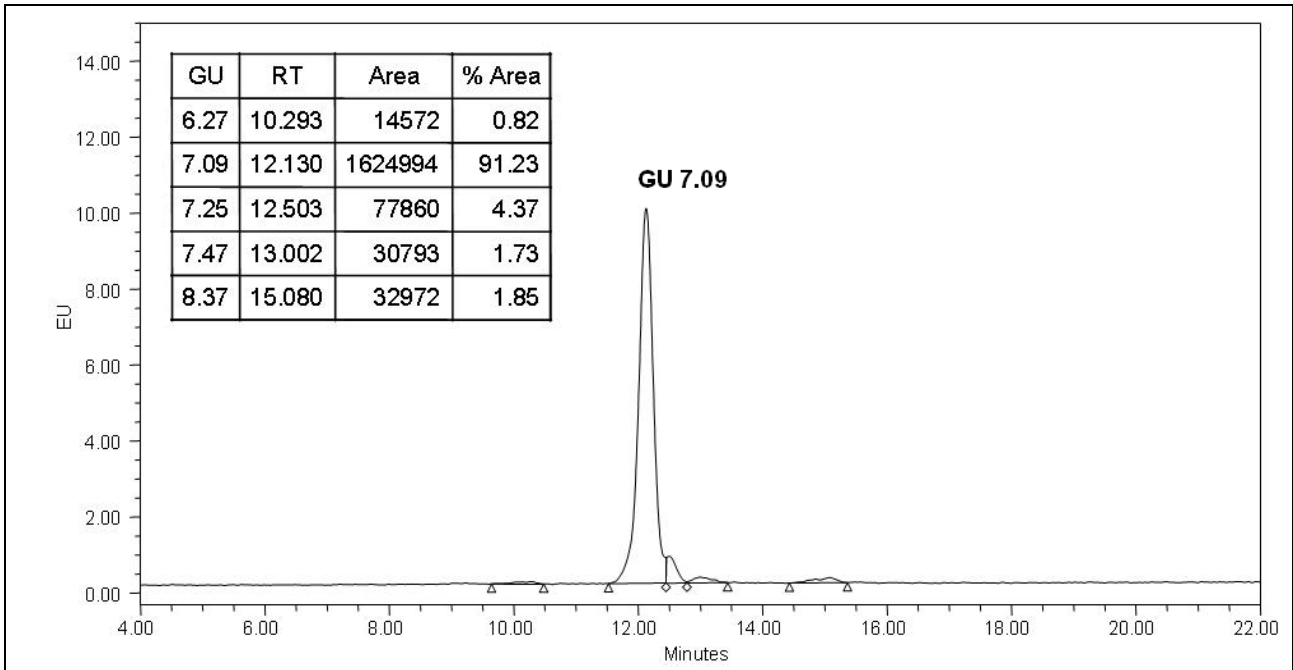
Figure 3: LudgerSepN2 chromatogram of 2AB labelled NA2 glycan (CN-NA2-10U, Batch B12N-01).
