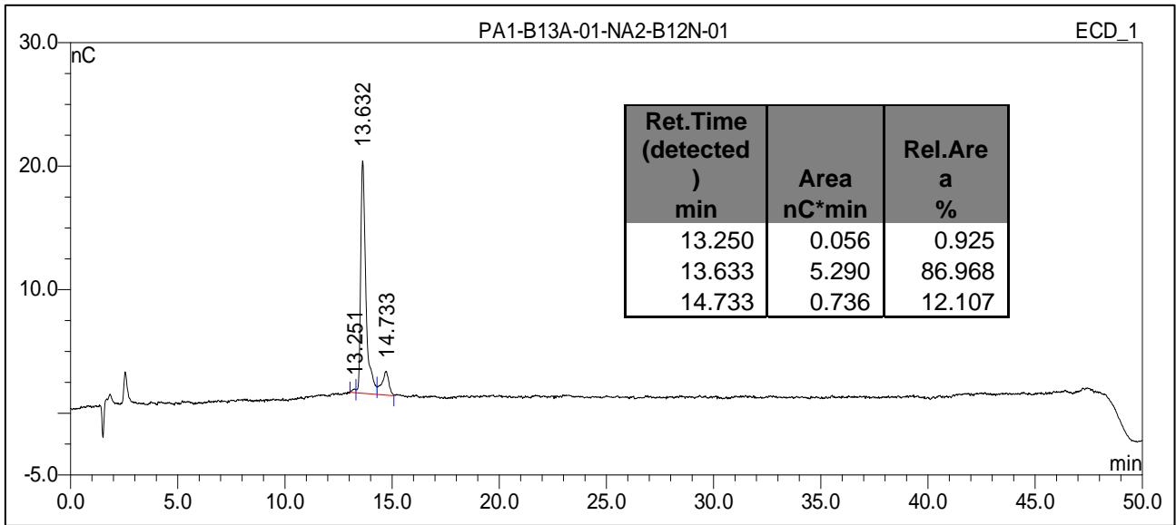
Figure 1: HPAE-PAD HPLC Profile of NA2 (CN-NA2-10U, Batch B12N-01).
