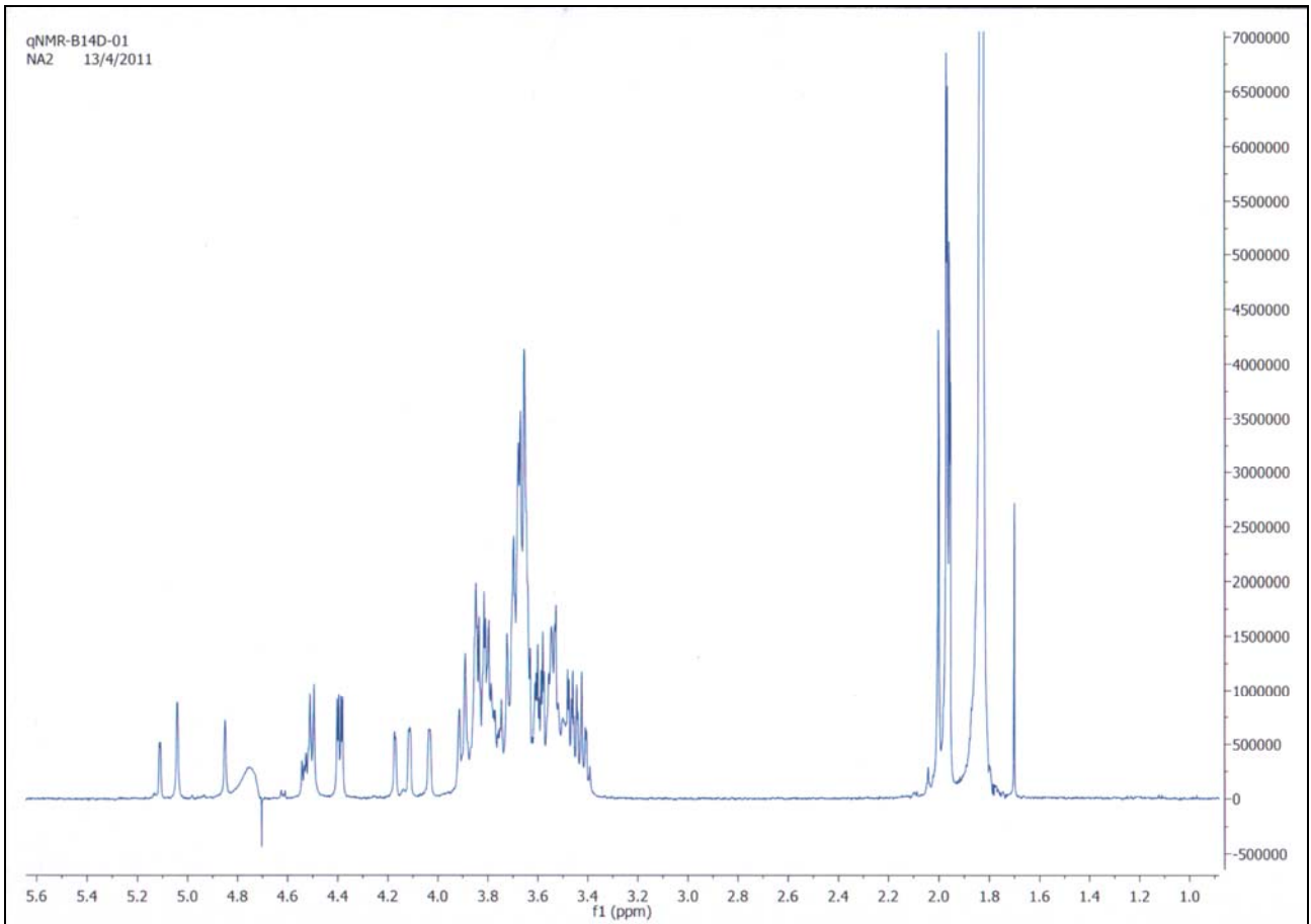
Figure 2: 500MHz 1 H-NMR of NA2 glycan BULK (CN-NA2-BULK Batch A9AQ-01).
