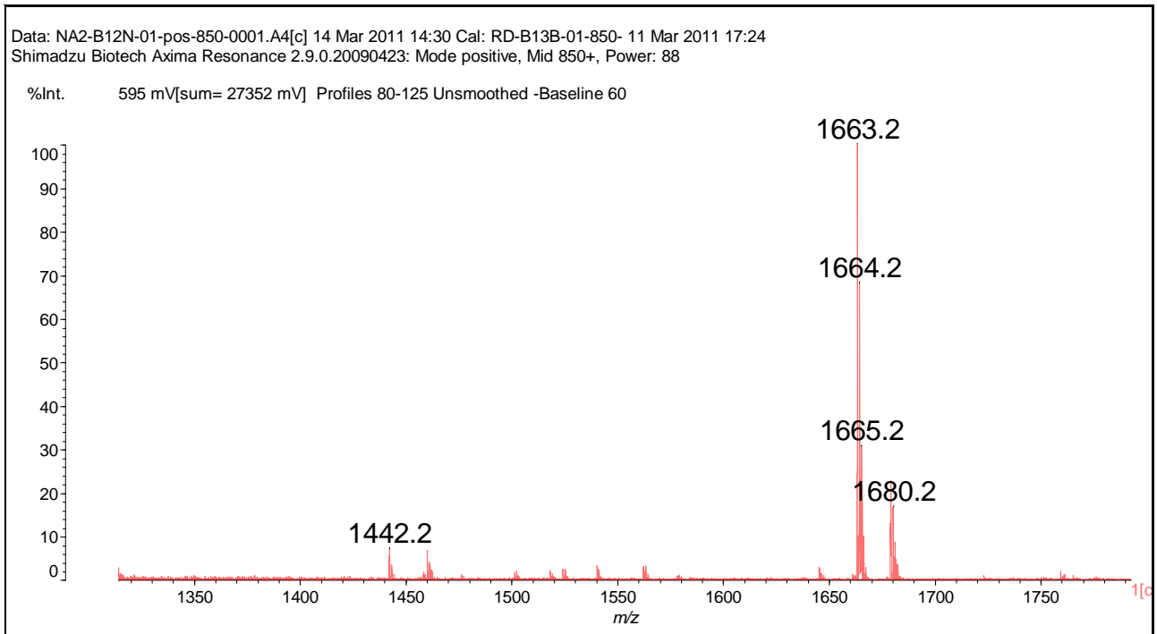
Figure 4: Positive ion mass spectrum of NA2 glycan (CN-NA2-10U, Batch B12N-01). Theoretical mass 1663.6Da [M+Na] + .
