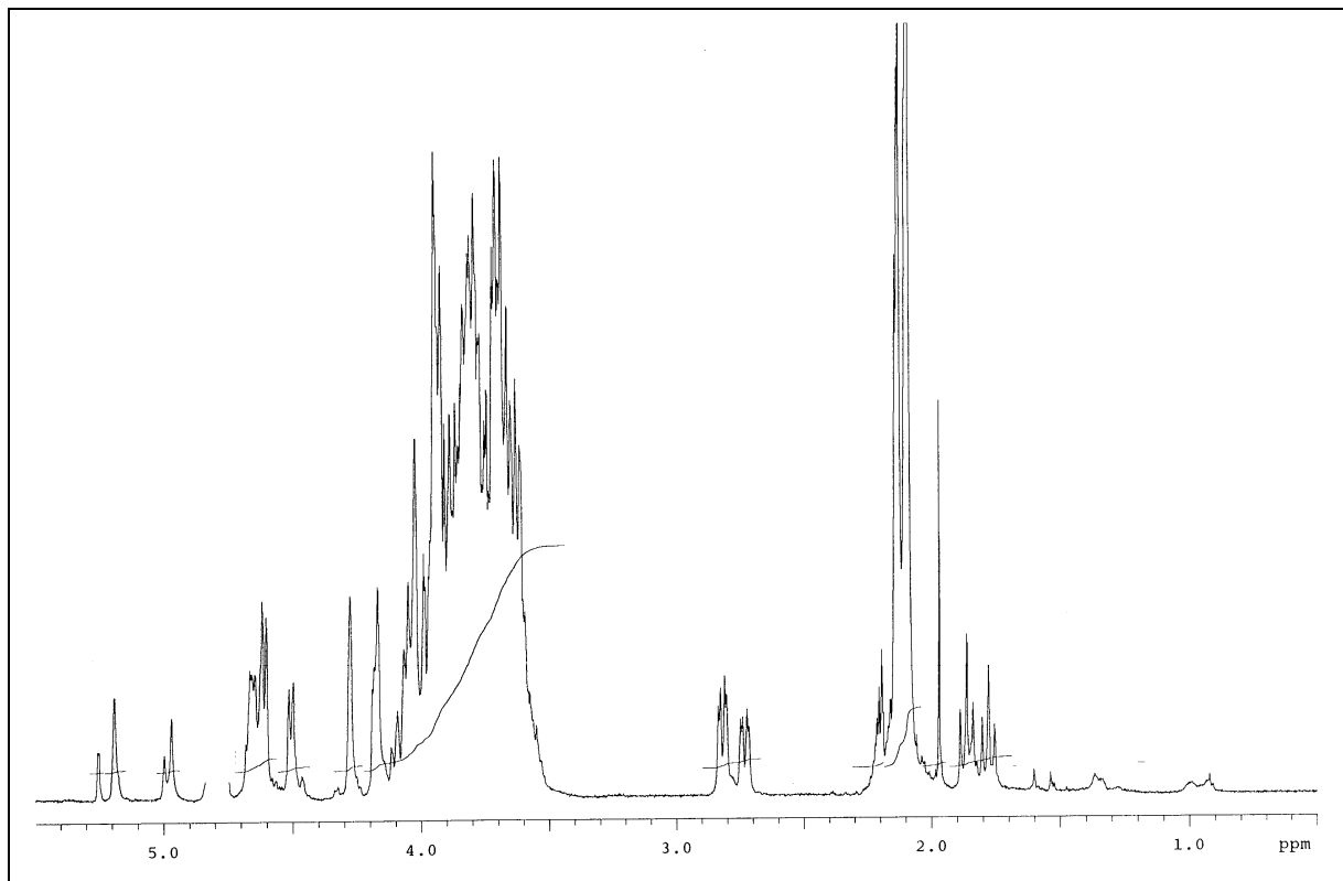
Figure 2: 500MHz 1 H-NMR of A3 glycan BULK (CN-A3-BULK Batch A34T-01).
