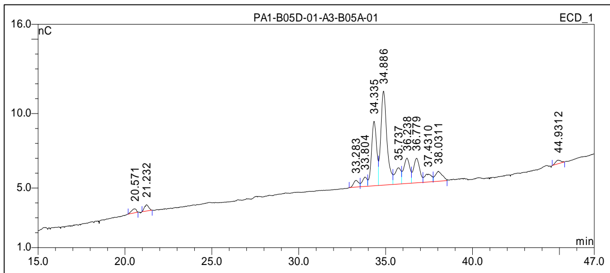
Figure 1 : HPAE-PAD HPLC Profile of A3 (CN-A3-10U, Batch B05A-01).
