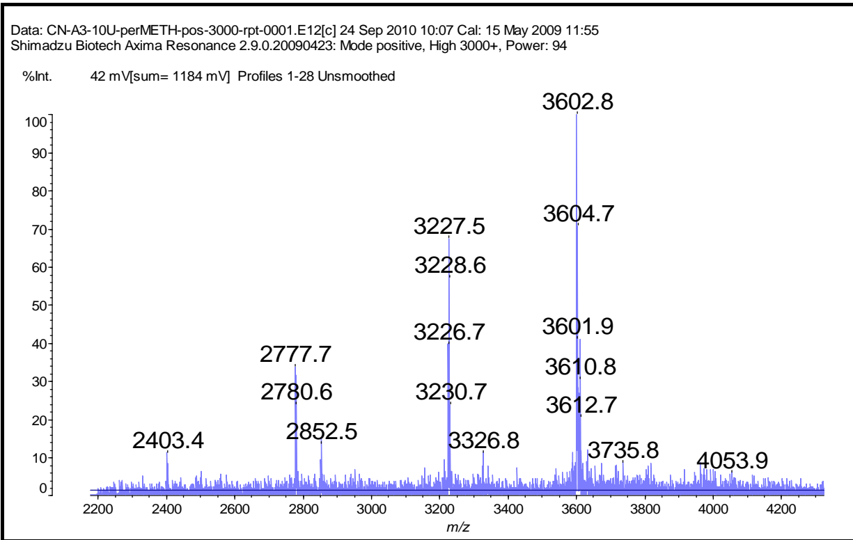
Figure 4: Positive ion mass spectrum of permethylated A3 glycan (CN-A3-10U, Batch B05A-01). Theoretical mass 3602.8 Da [M+Na]^+ .
