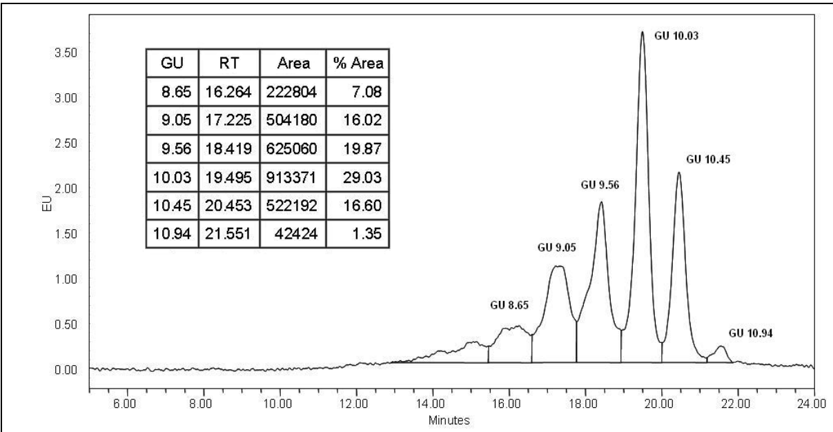
Figure 3: LudgerSepN2 chromatogram of 2AB labelled A3 glycan (CN-A3-10U, Batch B05A-01).
