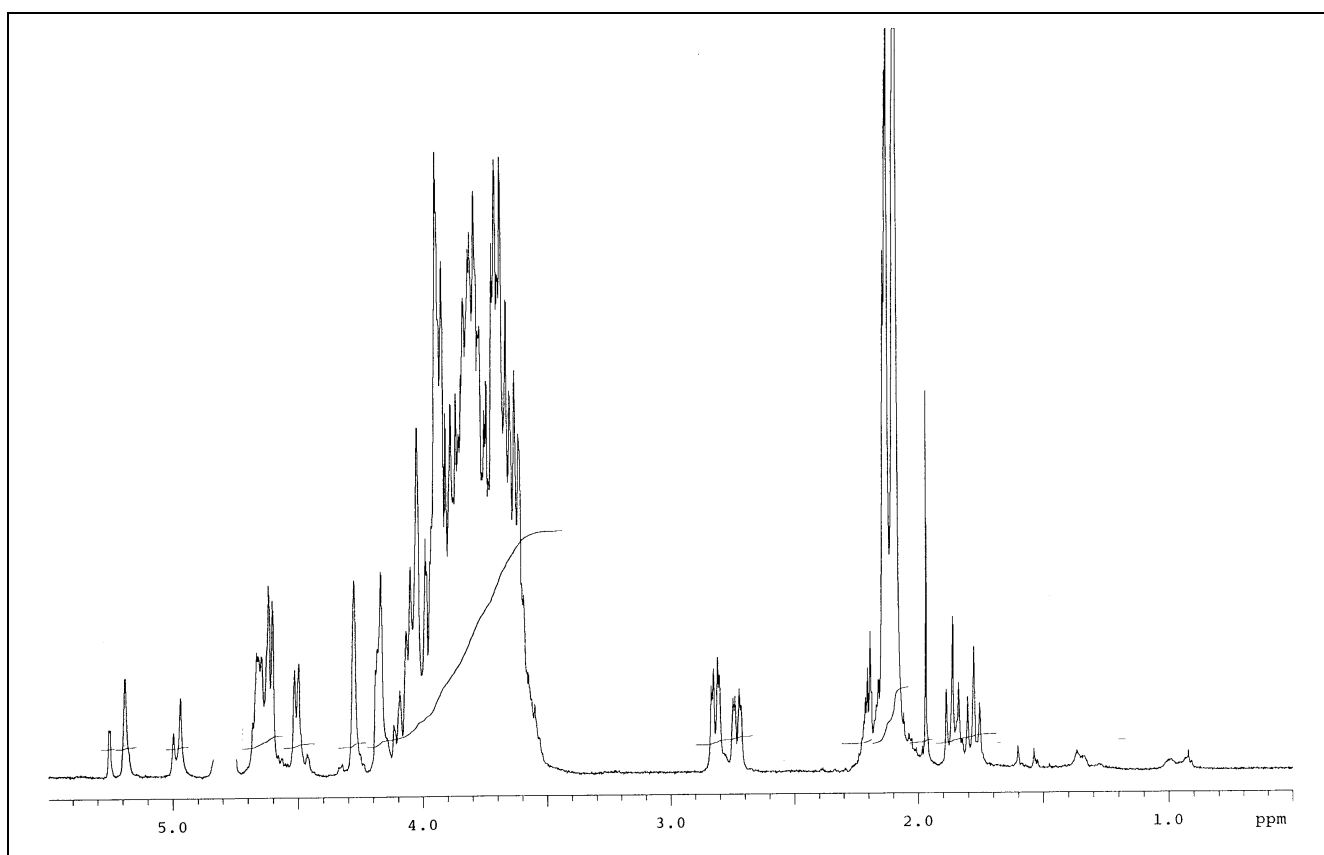
Figure 1 : 500 MHz ^1\text{H-NMR} of A3 Glycan (Cat. No.CN-A3-10U, Lot No. A34T-02)
