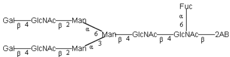
Text Notation
