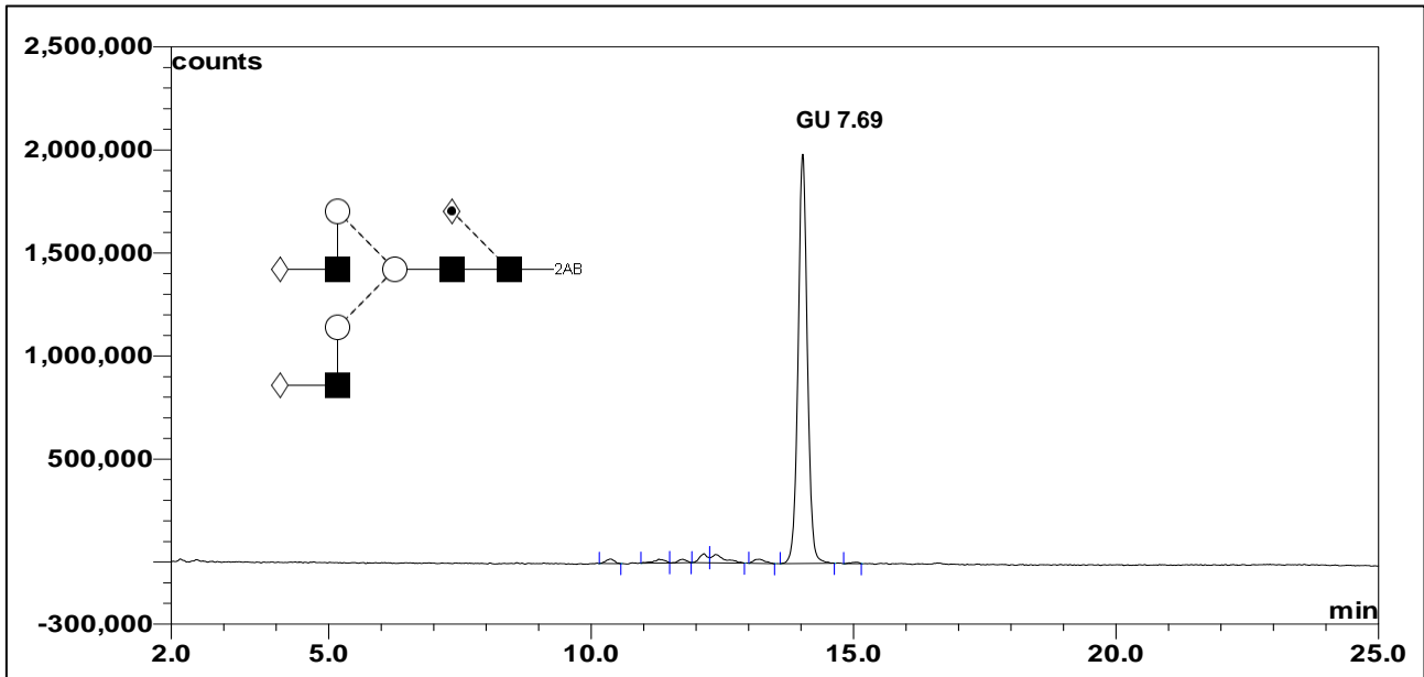
Figure 1: LudgerSepN2 HPLC profile of 2AB labeled NA2F glycan (Cat. #: CAB-NA2F-01, Batch B17M-05).
