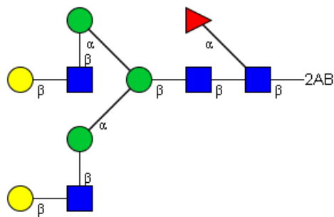
CFG Notation
