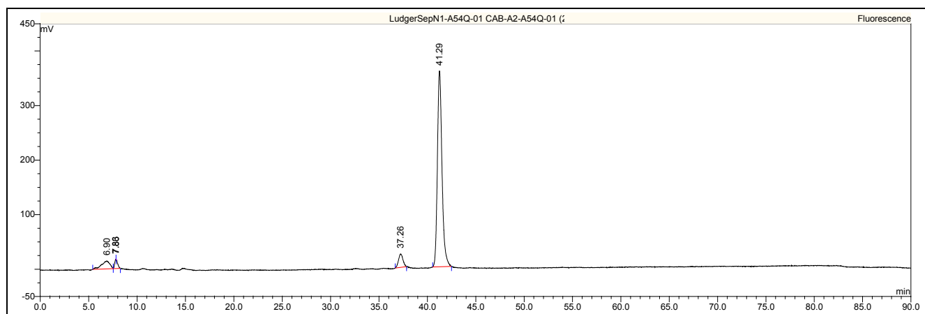
Figure 1 : LudgerSepN1 HPLC profile of 2AB labeled A2 glycan (Cat. #: CAB-A2-01, Lot No. A54Q-01).
