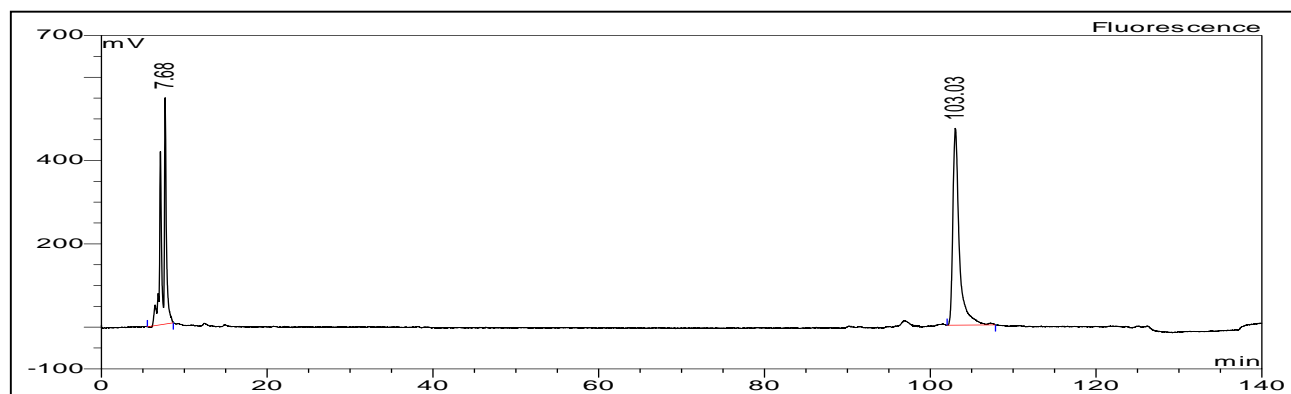
Figure 1 : LudgerSepN1 HPLC profile of 2AB labeled MAN-8 glycan (Cat. #: CAB-MAN8-01, Lot No. A81M-02). Free dye peak at 7.68 minute; CAB-MAN8-01 peak seen at 103.03, under the following conditions.
