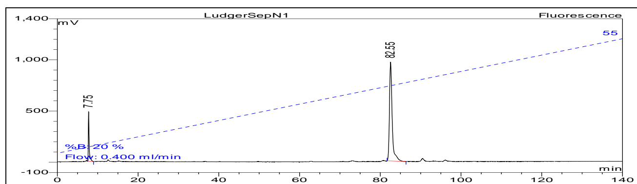
Figure 1 : LudgerSepN1 HPLC profile of 2AB labeled MAN-5 glycan (Cat. #: CAB-MAN5-01, Lot No. A817-02). Free dye peak at 7.75 minute; CAB-MAN-5 peak seen at 82.55, under the following conditions.
