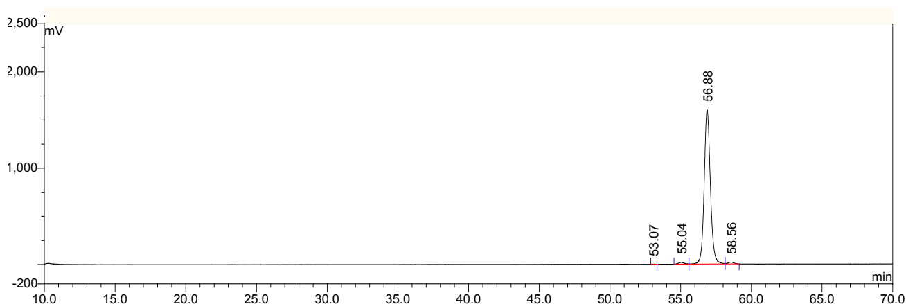
Figure 1 : LudgerSep N1 HPLC Column (Cat. No. LS-N1-4.6x250) profile of CAB-GLC17-1 Lot # A46F-03
