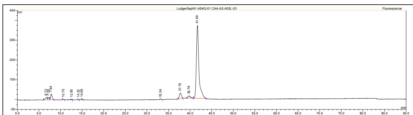
Figure 1 : LudgerSepN1 HPLC profile of 2AA labeled A2 glycan (Cat. #: CAA-A2-01, Lot No. A53L-03).
