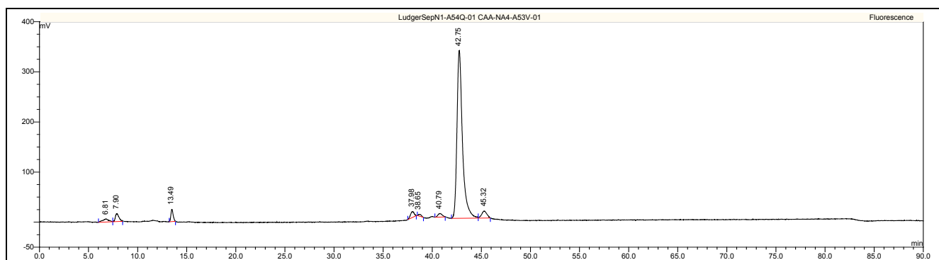
Figure 1 : LudgerSepN1 HPLC profile of 2AA labeled NA4 glycan (Cat. #: CAA-NA4-01, Lot No. A53V-01).
